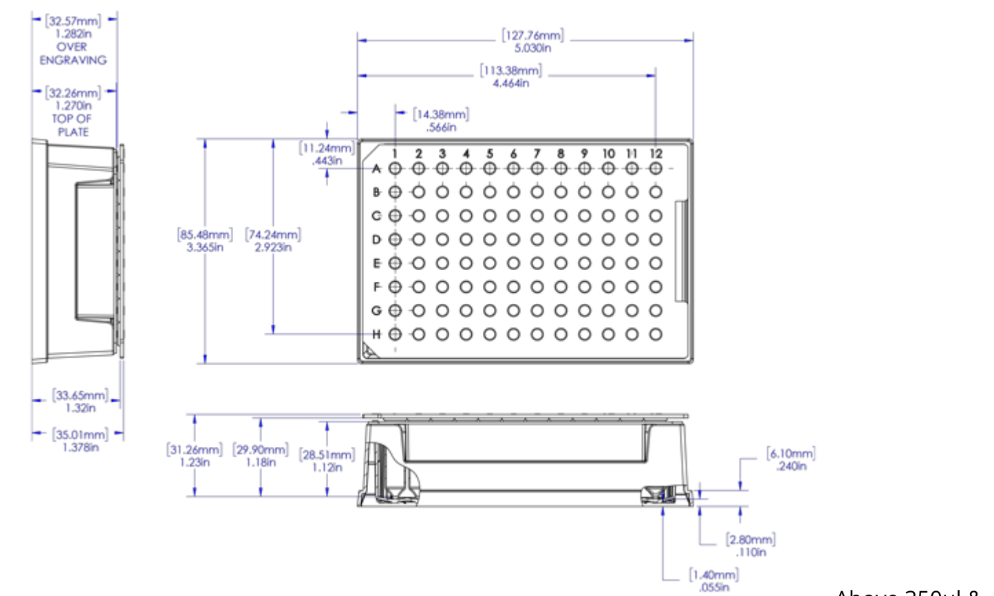
500ul dimension drawing for U-2D system
